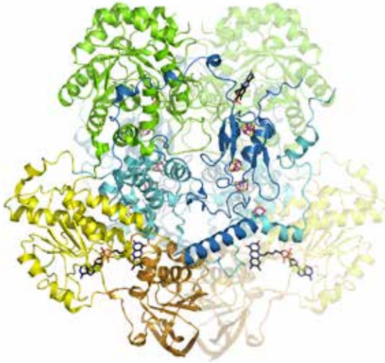
Tredimensionella strukturen hos dihydropyrimidin dehydrogenase. Bild: Centre of Cellular Imaging i Göteborg, courtesy of Doreen Dobritzsch and Gunter Schneider.
